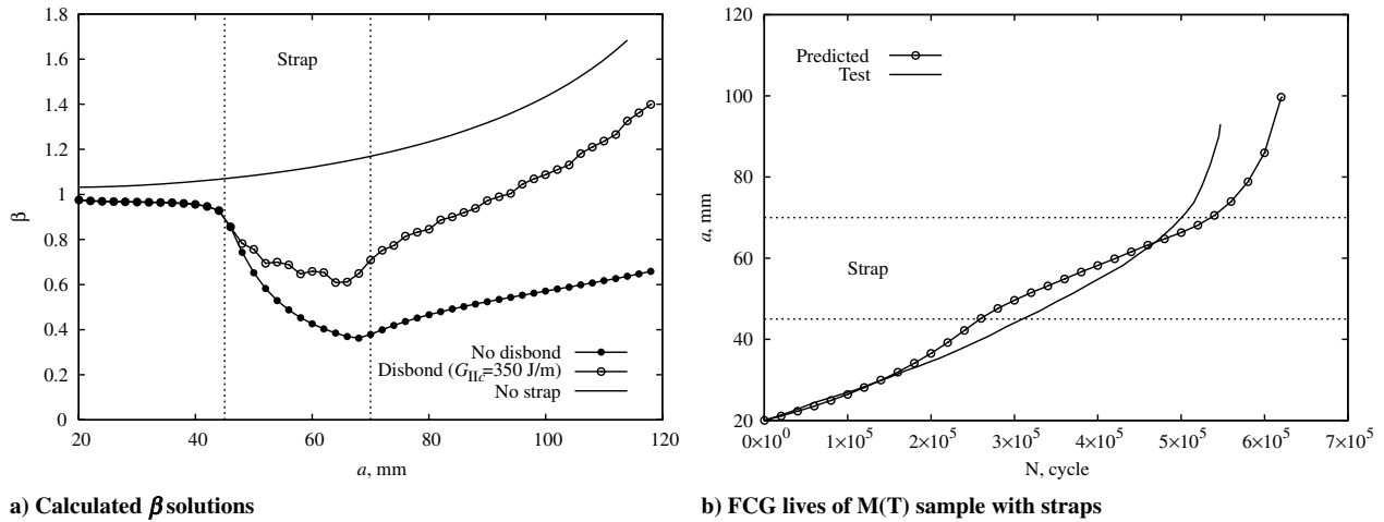
Fig. 5 M(T) sample with and without straps; test [6] and predicted results.
