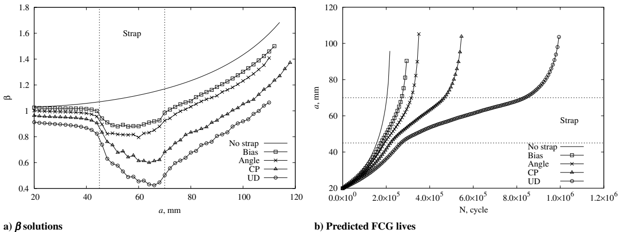
Fig. 7 Comparison of different carbon-epoxy strap layup configurations attached to the M(T) sample. Layup patterns: UD [0] 4 , CP [90/0] 4 , angle [30/60] 4 , bias [−45/45] 4 .
