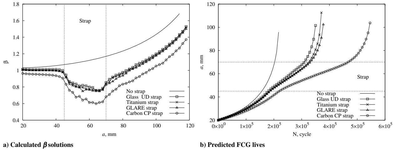
Fig. 8 Comparison of different strap materials. M(T) sample.
